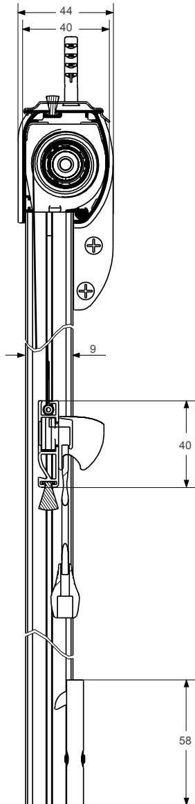
Vertical Section
