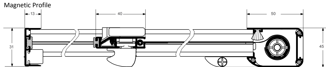
Horizontal Section
