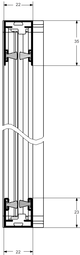
Vertical Section
