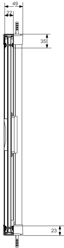
Vertical Section
