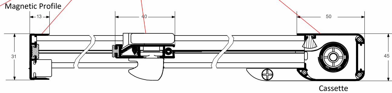
Horizontal Section
