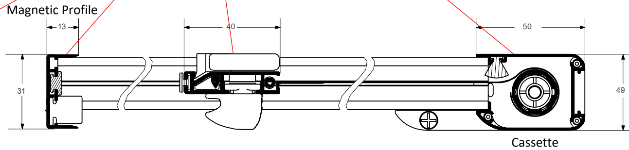
Horizontal Section
