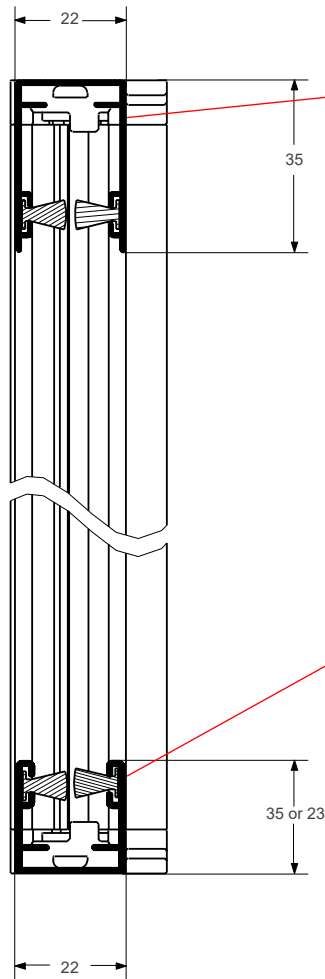
Vertical Section
