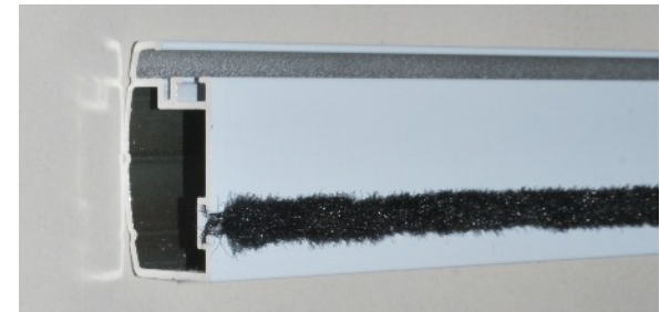
Integral brush pile in the profiles to create a seal with the door.
